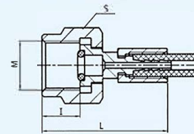
4. Direct connect to pressure gauge: HF P※ Unit: mm
