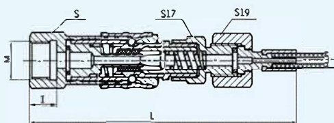
7. Snap-check fitting: HF S※ Unit: mm
