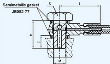
1. Adjustable fitting: HF J※ Unit: mm
